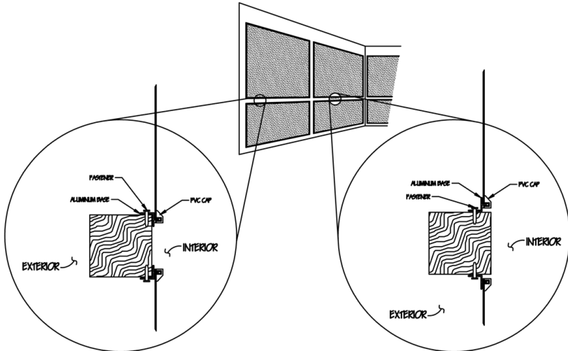
FLUSH MOUNT DETAIL SEE DRAWING DETAILS FOR FURTHER INFORMATION
